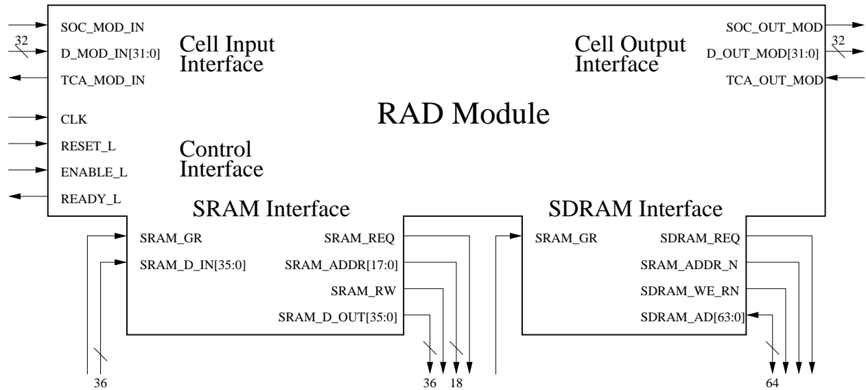
Figure 1: RAD Module Interface
