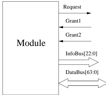
Figure 7: Module Interface for the SDRAM access
