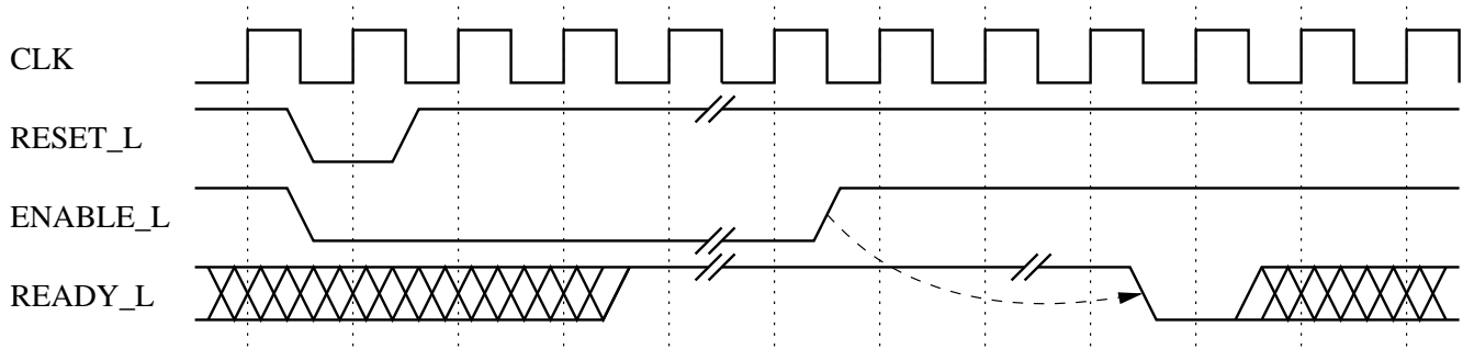
Figure 2: Timing diagram for Control Interface
