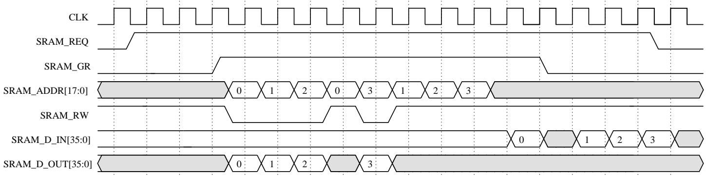
Figure 6: Module timing diagram for SRAM Interface. Note that this diagram uses a point of reference from inside the module and assumes that all signals are flopped at the module boundary.
