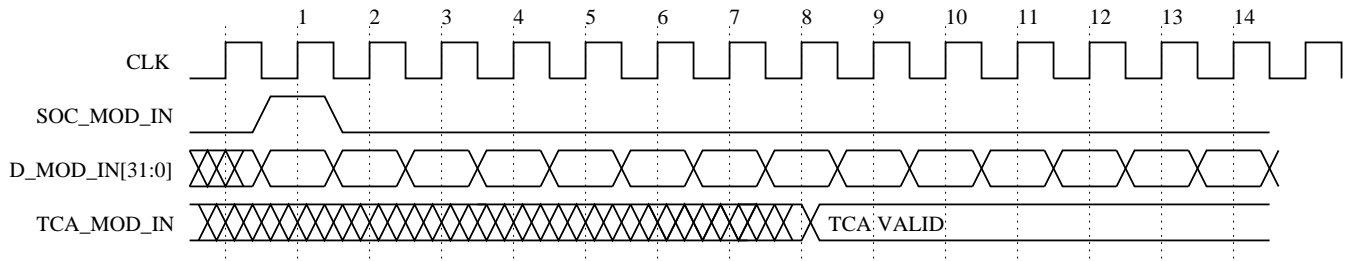
Figure 3: Timing diagram for Cell Input Interface.
