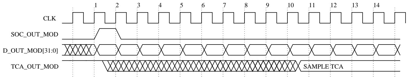
Figure 4: Timing diagram for Cell Output Interface.
