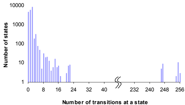
Figure 6. Distribution of number of transitions per state in the D 2 FA constructed from the Cisco590 expression set
